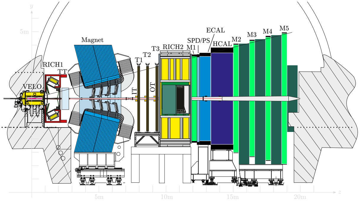
Figure 6.2. Side view of the LHCb detector. Adapted from [238; 239].
